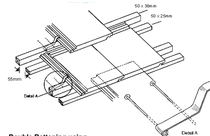
Double Battening using Double Battening Clip (9204)
