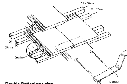
Double Battening using Double Battening Clip (9204)
