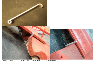
Tile Clip and Nails (9246 and 9333)
